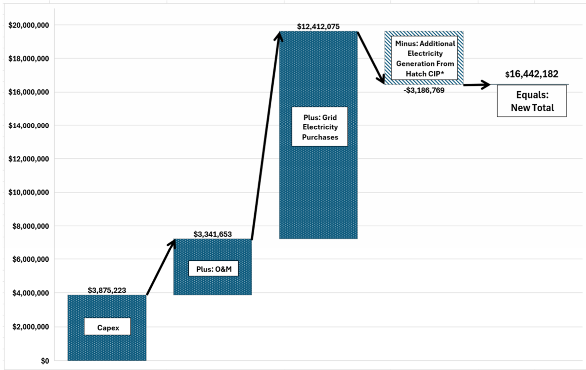
Figure 7: Detailed Energy Costs for Craggy Dam Scenario 1
